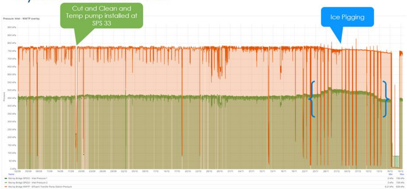
FIGURE 7: SCADA SHOWING PIPE PRESSURES
